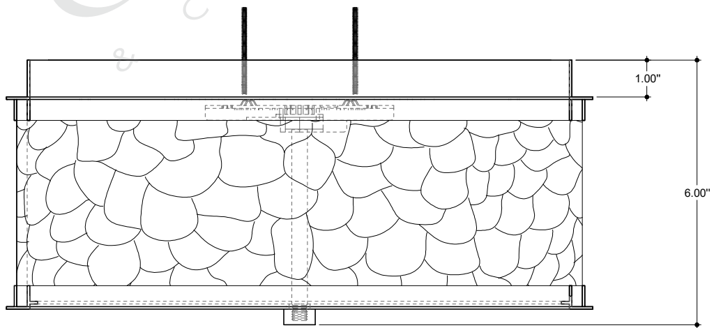
FRONT VIEW
